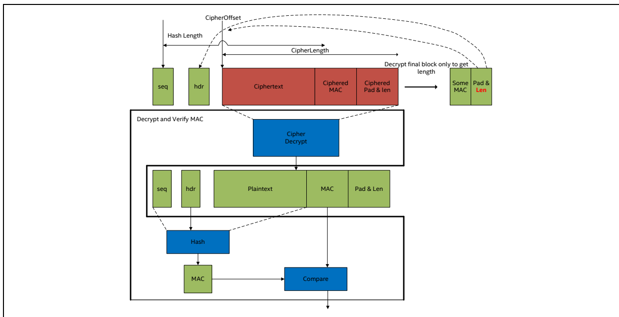
Figure 8. Secure Sockets Layer Inbound
