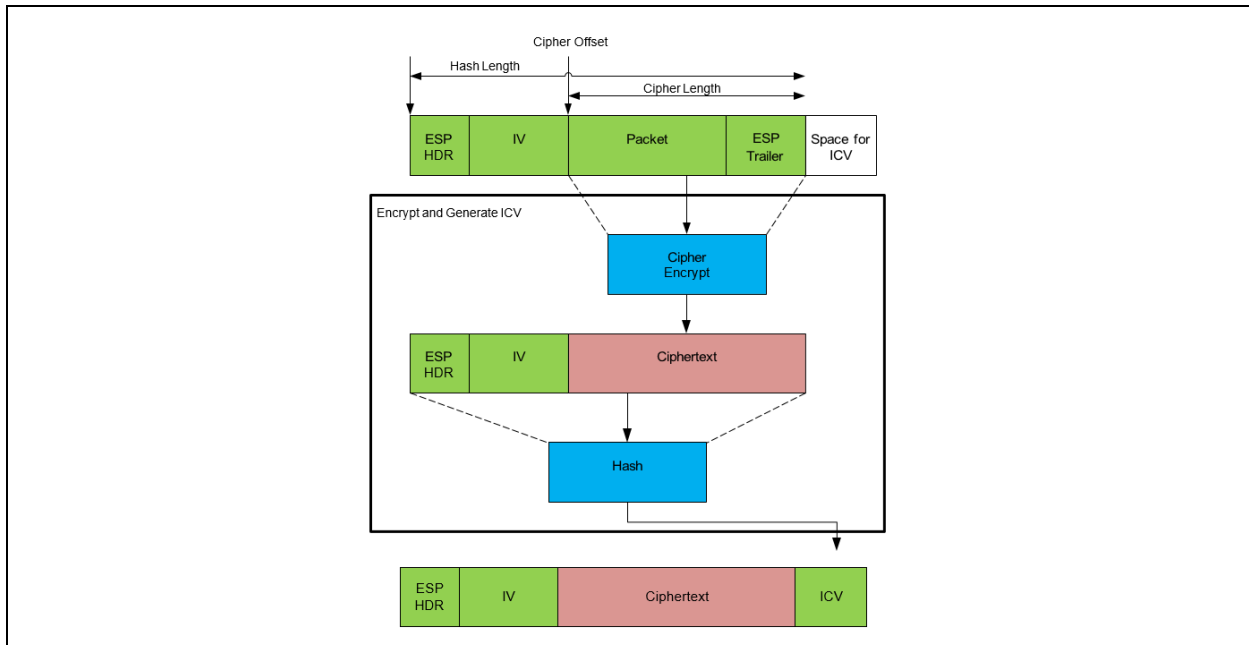
Figure 5. IPsec Outbound
