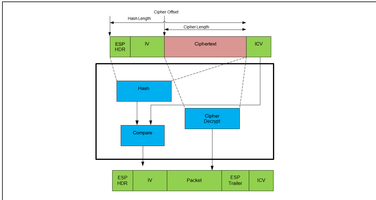
Figure 6. IPsec Inbound
