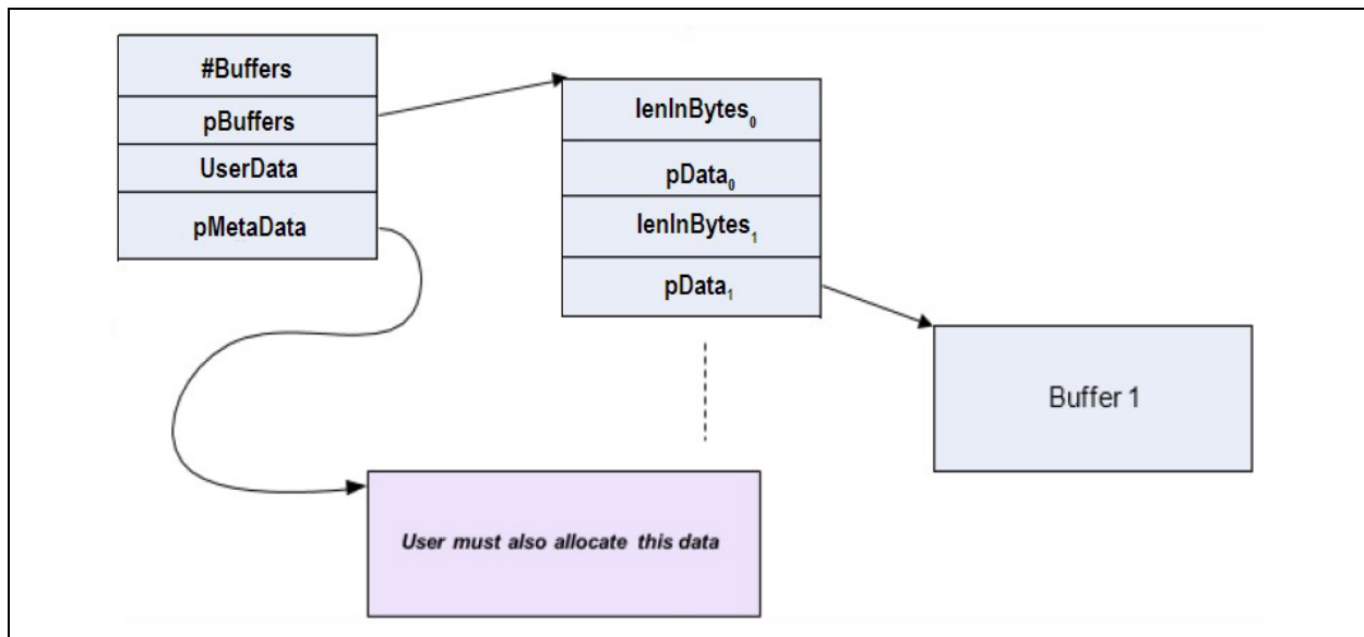
Figure 2. Scatter-Gather List Diagram
