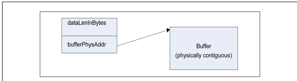
Figure 1. Flat Buffer Diagram
