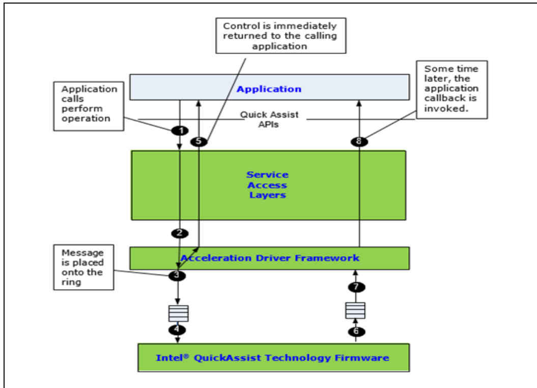
Figure 3. Asynchronous Operation
