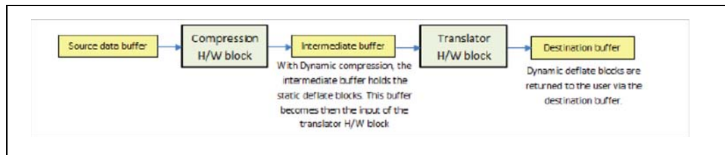
Figure 4. Dynamic Compression Data Path
